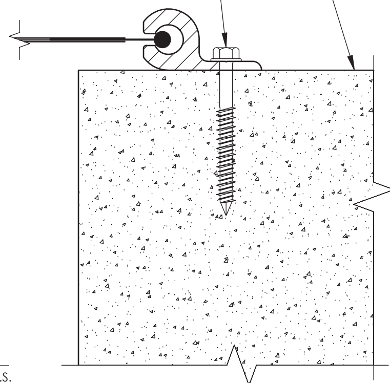
8 WALL MOUNT - SECTION
