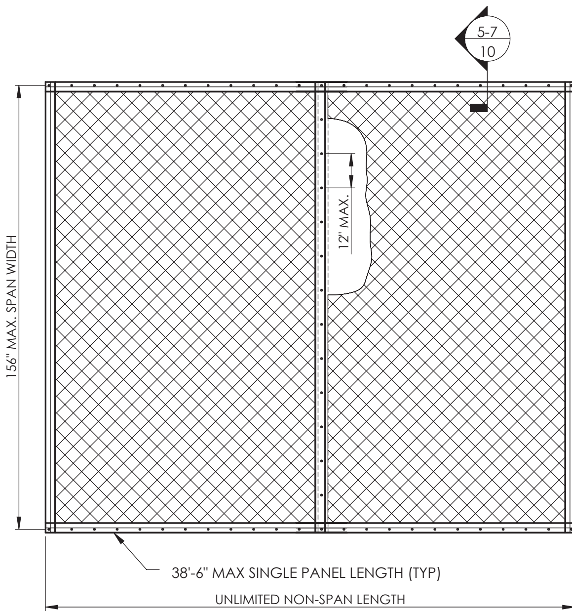
3 10 GROMMET SCREEN MULTIPLE PANEL - ELEVATION OPTIONAL COLUMN ATTACHMENT - VERTICAL OR HORIZONTAL INSTALLATION - N.T.S.
