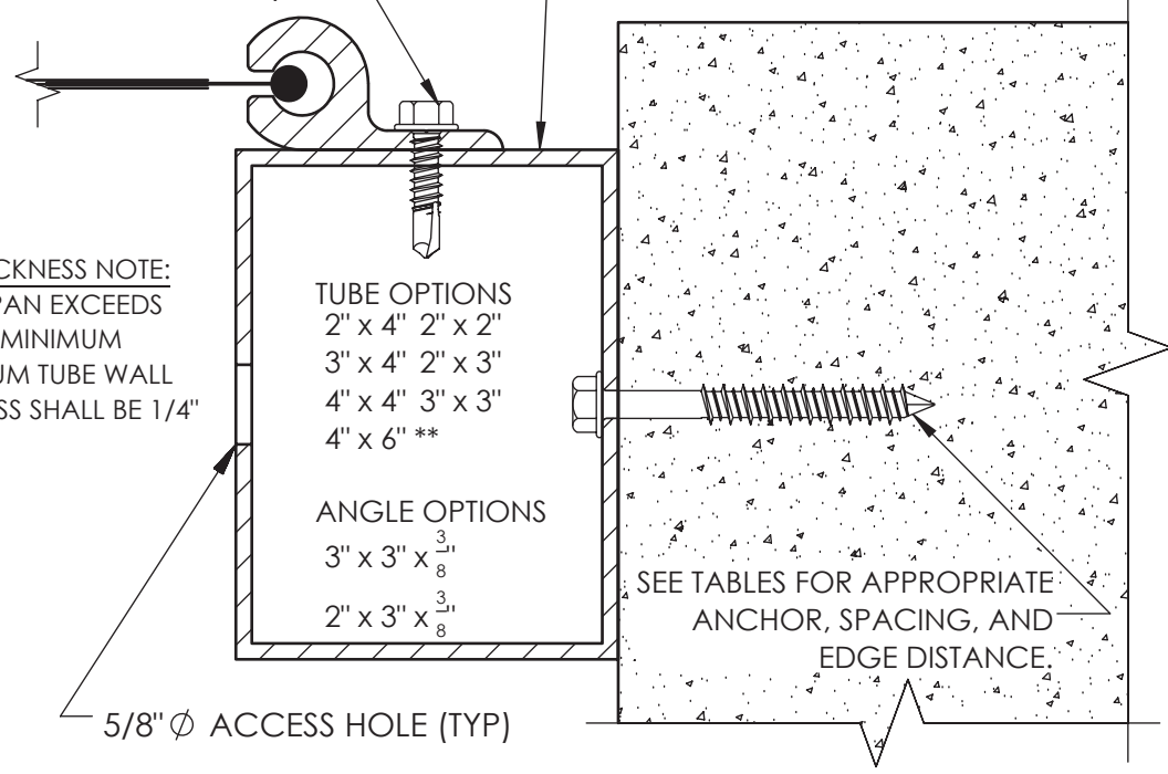
9 BUILD-IN MOUNT - SECTION
