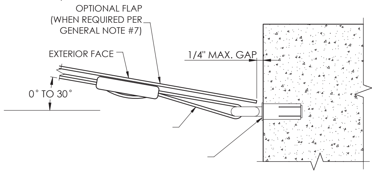
4 13 INSIDE MOUNT - SECTION EYE BOLT INSTALLATION (OPTION 4) - N.T.S. PLAN VIEW DETAIL
