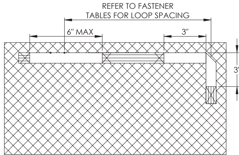
5 13 ALTERNATE FIXED STRAP/LOOP DETAIL STRUCTURAL ATTACHMENT FOR LOOP - N.T.S.: (3) ROWS STITCHING & BOX STITCH
