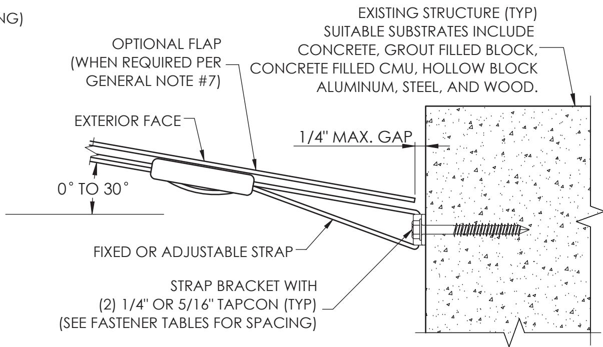
2 13 INSIDE MOUNT - SECTION STRAP BRACKET INSTALLATION (OPTION 2) - N.T.S. PLAN VIEW DETAIL
