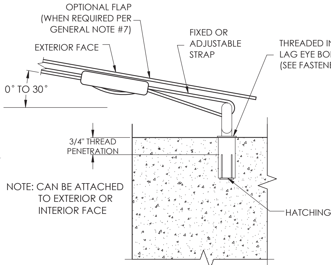
3 13 OUTSIDE MOUNT - SECTION EYE BOLT INSTALLATION (OPTION 3) - N.T.S. PLAN VIEW DETAIL
