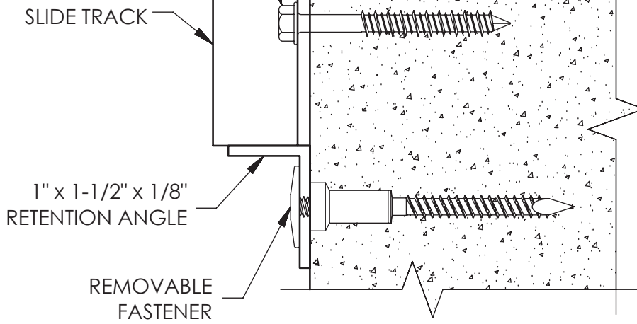
4 RETENTION ANGLE - SECTION (OPTIONAL)
