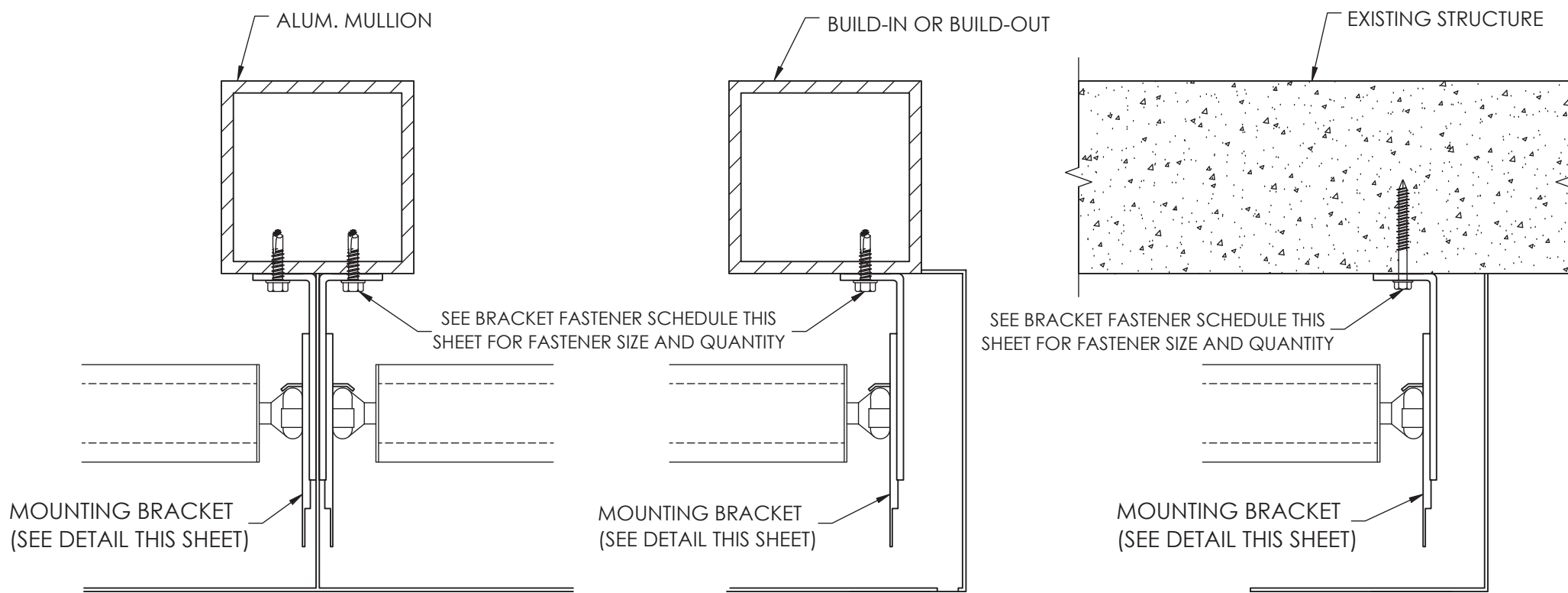
6 MOUNTING BRACKET INSTALLATION ROLL-UP SCREEN - N.T.S.
