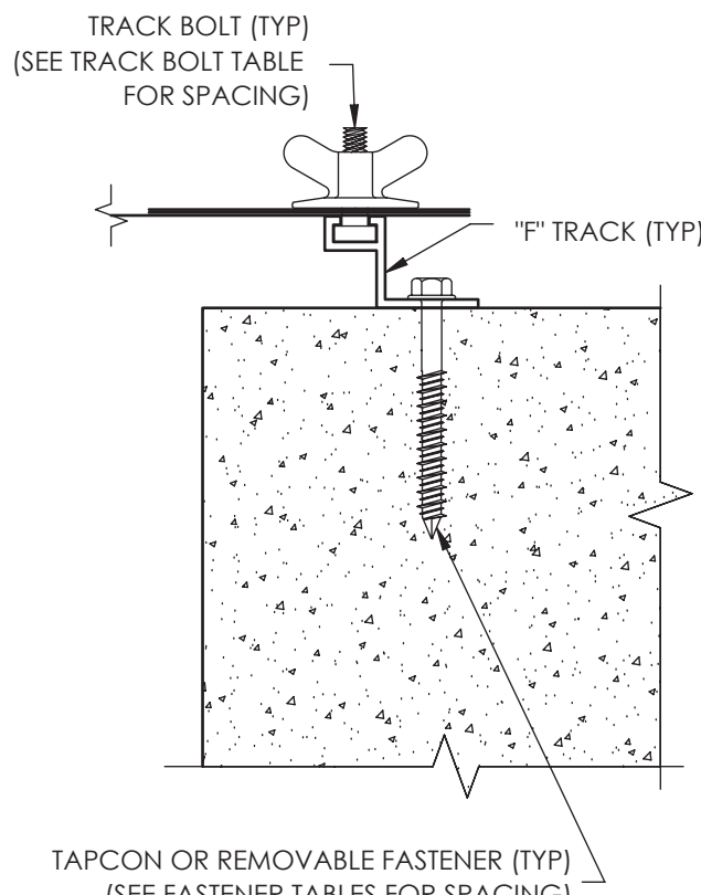
7 10 \"F\" TRACK MOUNT - SECTION STANDARD OR BUILD-OUT INSTALLATION (OPTION 3) - N.T.S.
