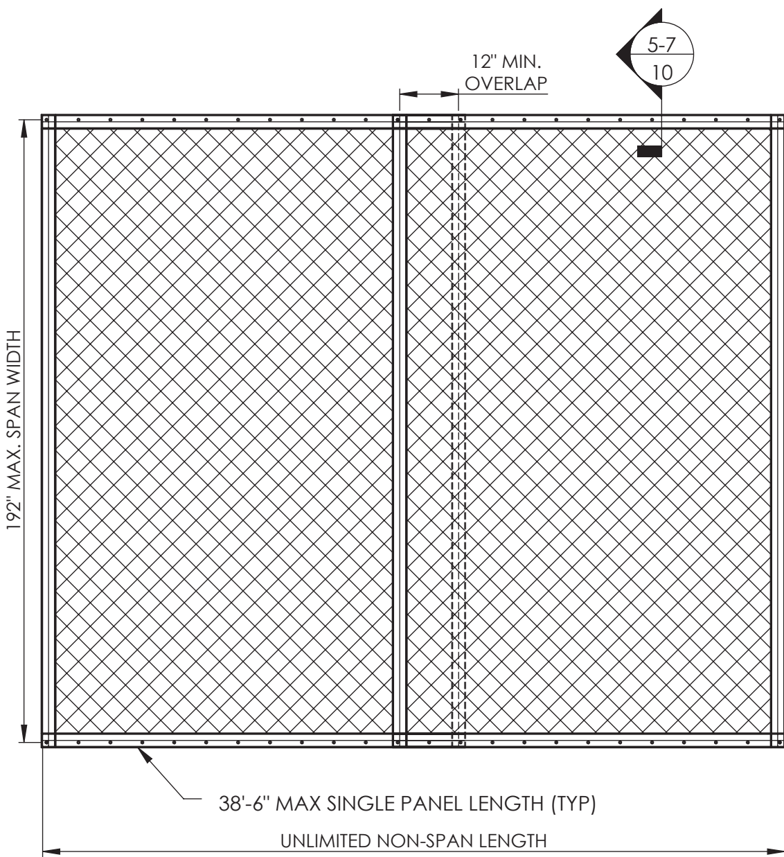
2 10 GROMMET SCREEN MULTIPLE PANEL - ELEVATION LAPPED SCREEN - VERTICAL OR HORIZONTAL INSTALLATION - N.T.S.
