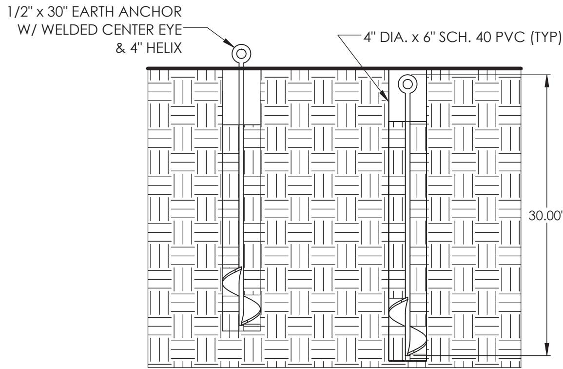
6 13 EARTH ANCHOR DETAIL EARTH ANCHOR INSTALLATION - N.T.S. SOIL CLASS 4A MEDIUM DENSE SAND
