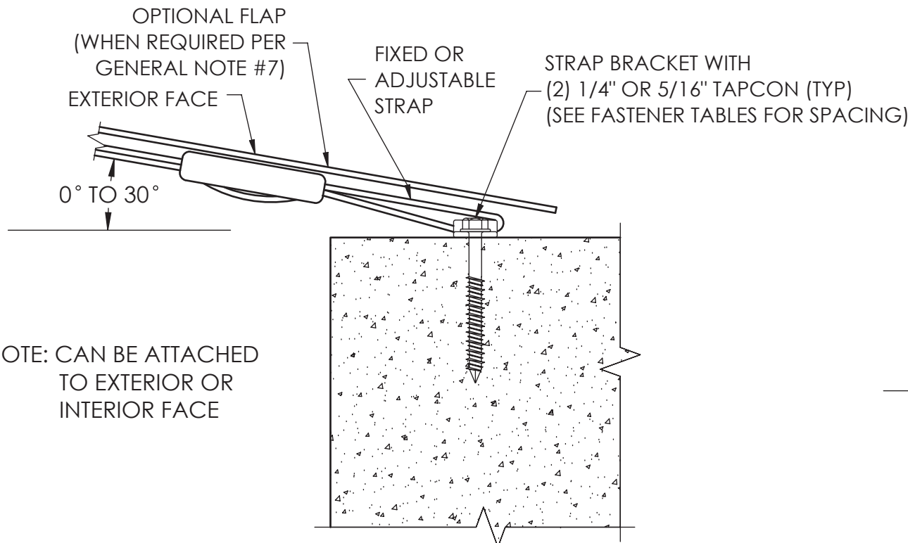
1 13 OUTSIDE MOUNT - SECTION STRAP BRACKET INSTALLATION (OPTION 1) - N.T.S. PLAN VIEW DETAIL
