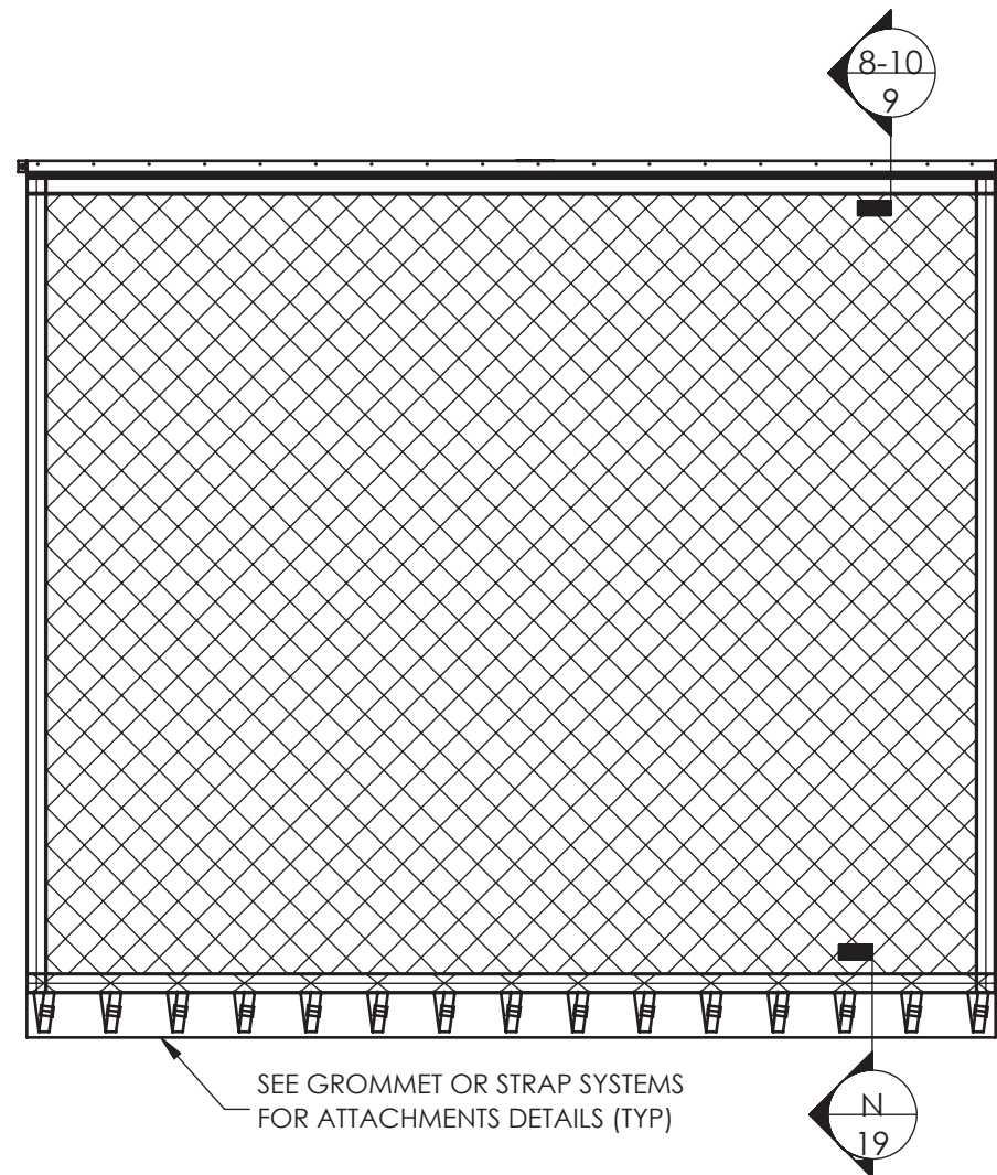
7 EASY SCREEN SINGLE PANEL - ELEVATION TYPICAL 2 SIDED ATTACHMENT - VERTICAL OR HORIZONTAL INSTALLATION - N.T.S.
