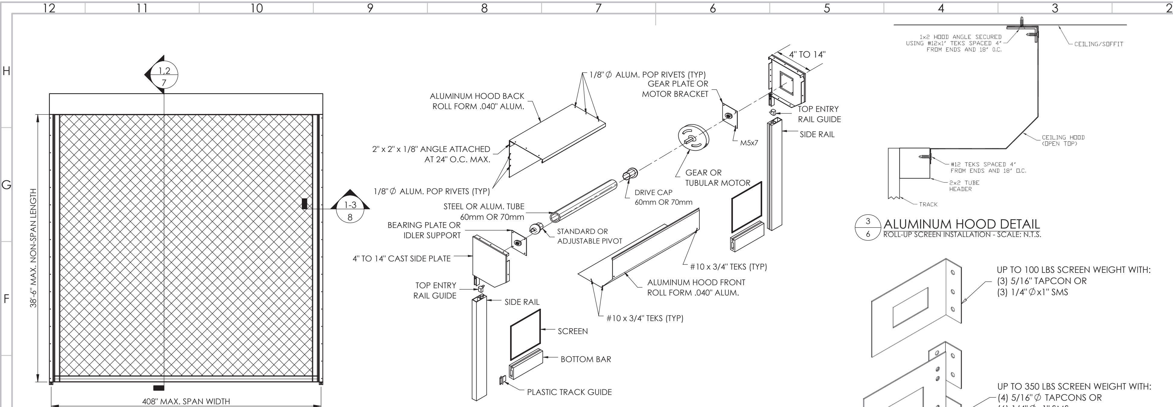
1 ROLL-UP SCREEN SINGLE PANEL - ELEVATION TYPICAL SINGLE SPAN UP TO 34'-0" INSTALLATION - N.T.S.
