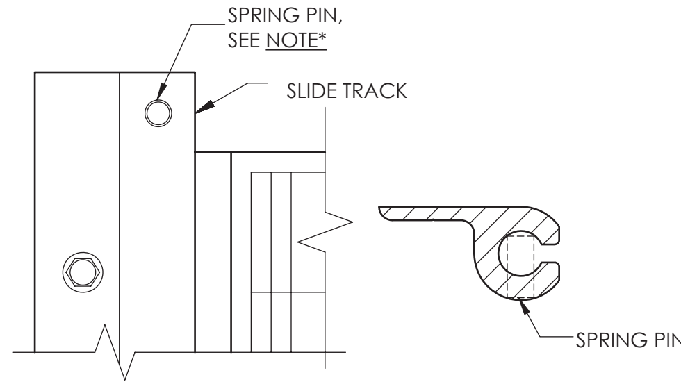
6 STAINLESS STEEL SPRING PIN
