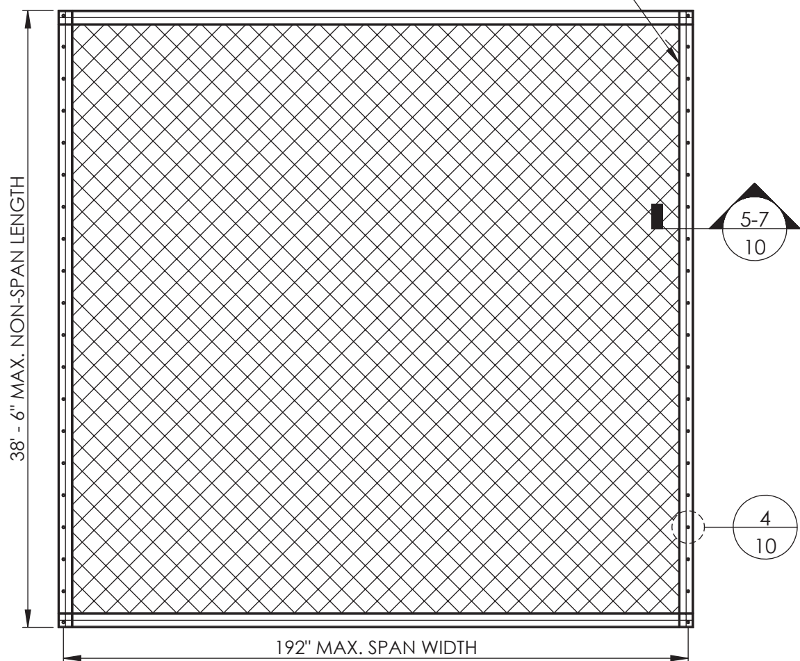
1 10 GROMMET SCREEN SINGLE PANEL - ELEVATION TYPICAL 2 SIDED ATTACHMENT - VERTICAL OR HORIZONTAL INSTALLATION - N.T.S.
