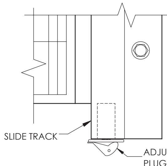
5 NEOPRENE ADJUSTABLE PLUG W/ BRASS FITTING
