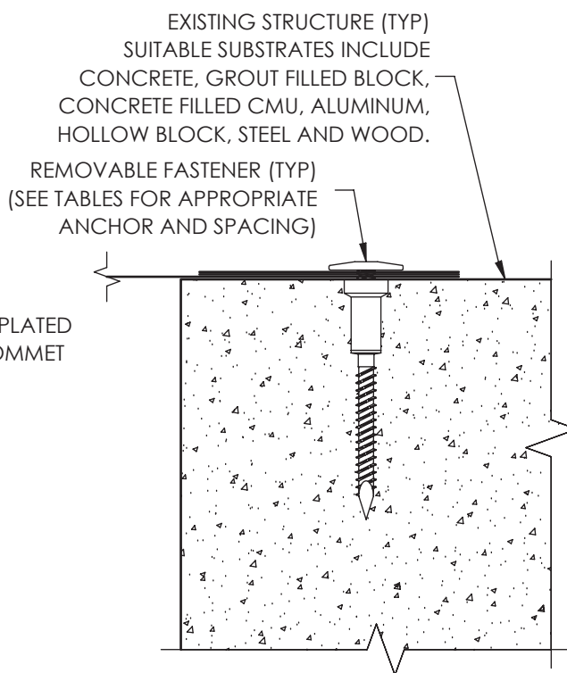
5 10 WALL MOUNT - SECTION TYPICAL INSTALLATION (OPTION 1) - N.T.S.
