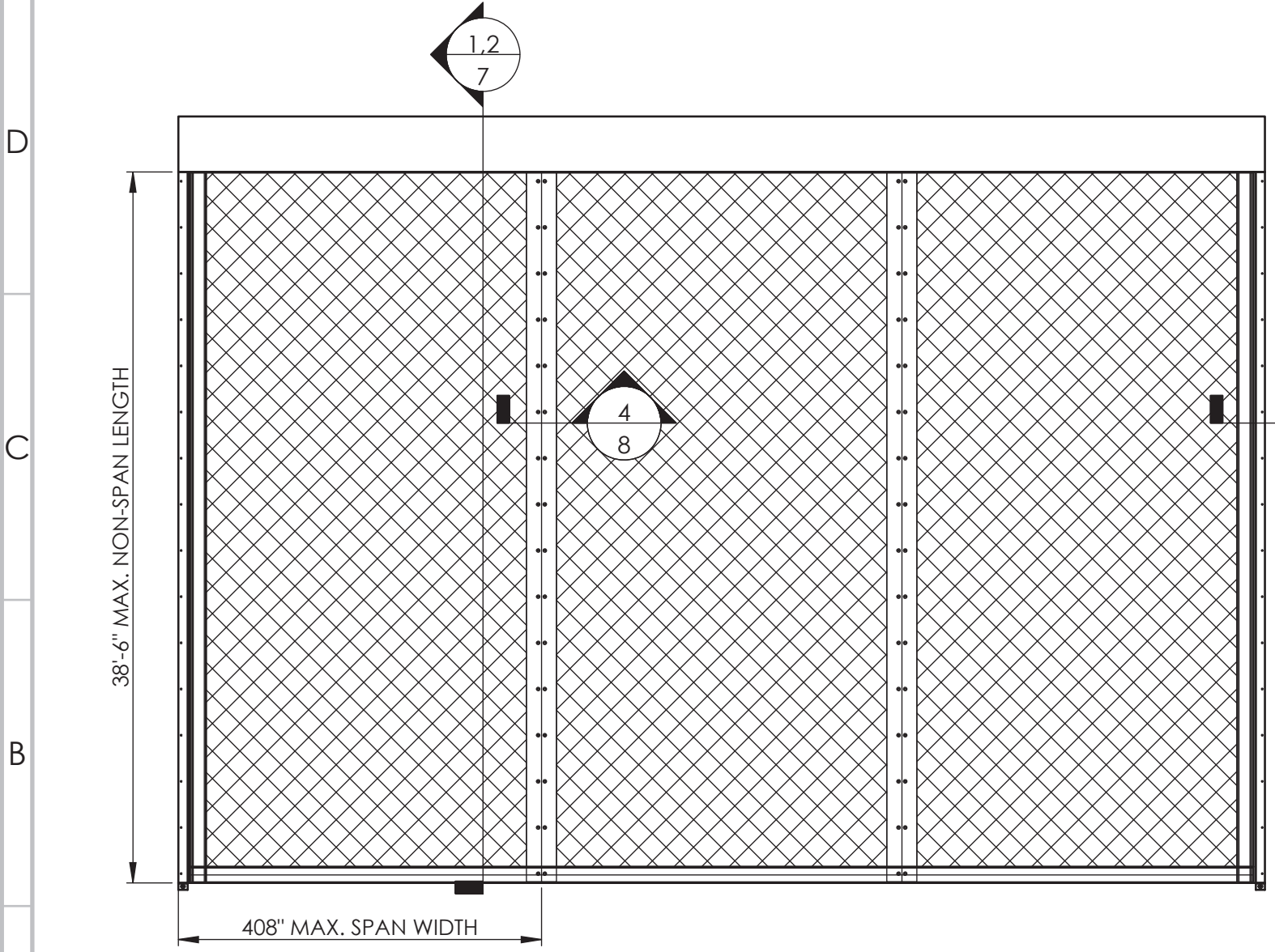
5 ROLL-UP SCREEN MULTIPLE UNIT - ELEVATION APPROVED INTERMEDIATE MULLION REQUIRED FOR INSTALLATION - N.T.S.
