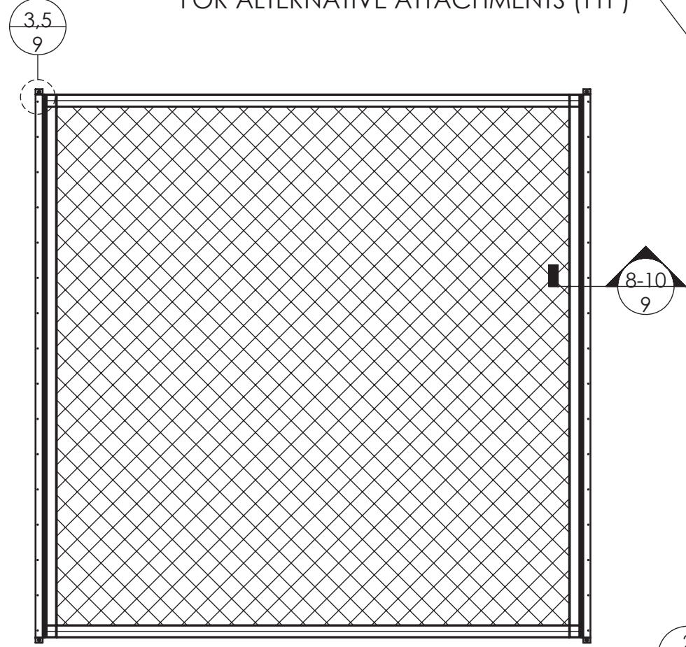
1 SLIDE SCREEN SINGLE PANEL - ELEVATION TYPICAL 2 SIDED ATTACHMENT - VERTICAL OR HORIZONTAL INSTALLATION - N.T.S.
