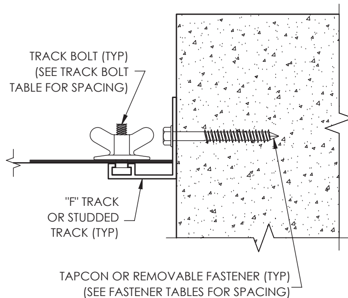
6 10 BUILD-IN MOUNT - SECTION ANGLED \"F\" OR STUDDED INSTALLATION (OPTION 2) - N.T.S.
